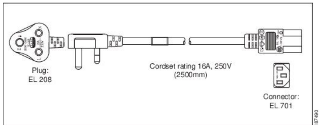
Figure 6: SFS-250V-10A-IS
