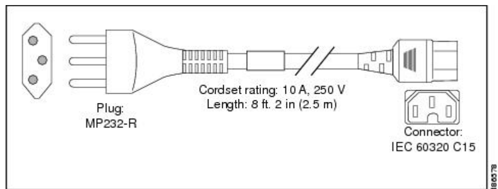
Figure 9: CAB-9K10A-UK
