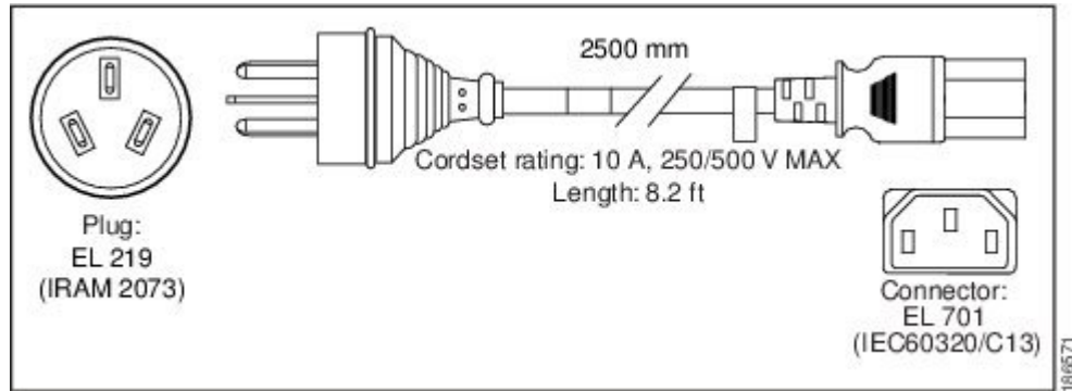
Figure 2: CAB-9K10A-AU
