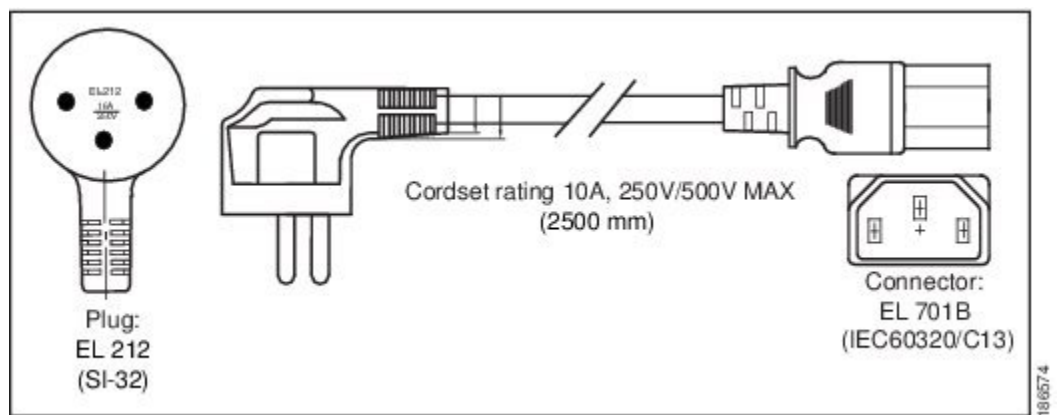
Figure 7: CAB-9K10A-IT
