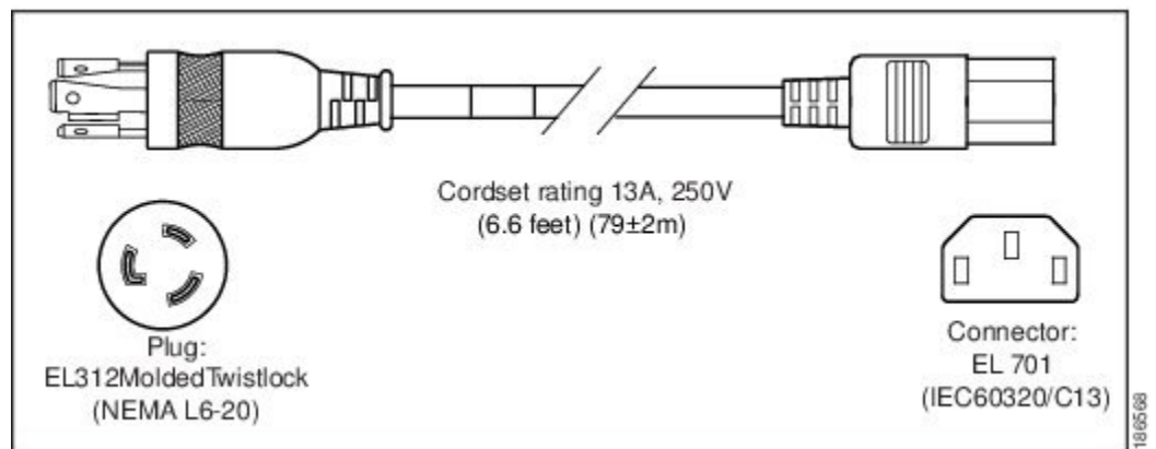
Figure 11: CAB-N5K6A-NA
