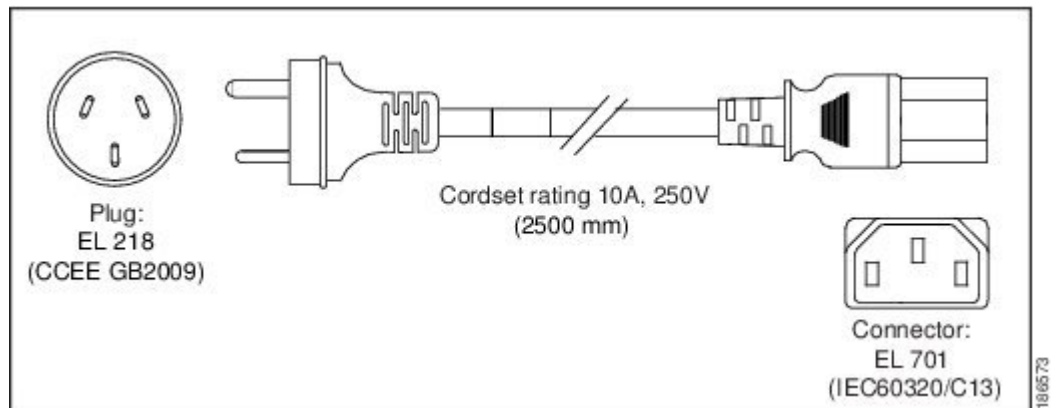
Figure 3: SFS-250V-10A-CN
