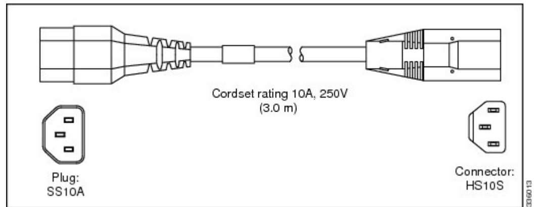
Figure 14: CAB-C13-C14-AC, Jumper Power Cord (3 m)
