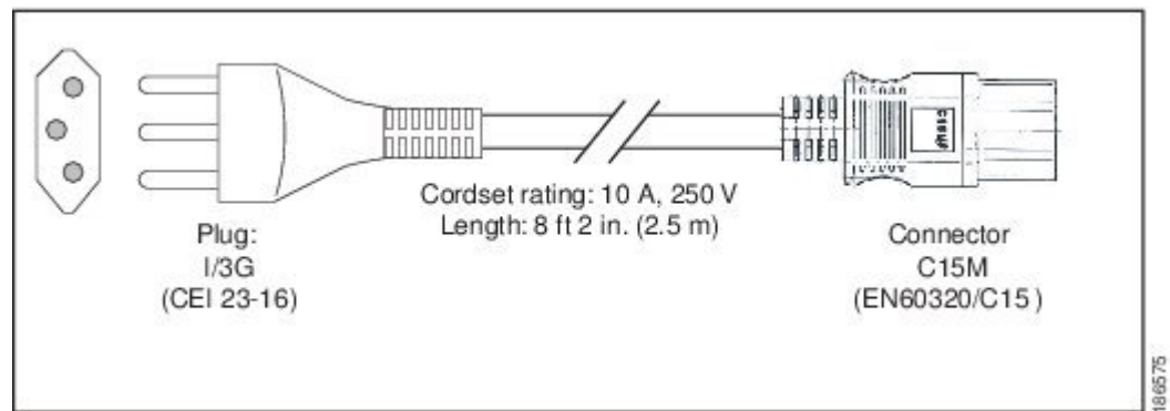
Figure 8: CAB-9K10A-SW
