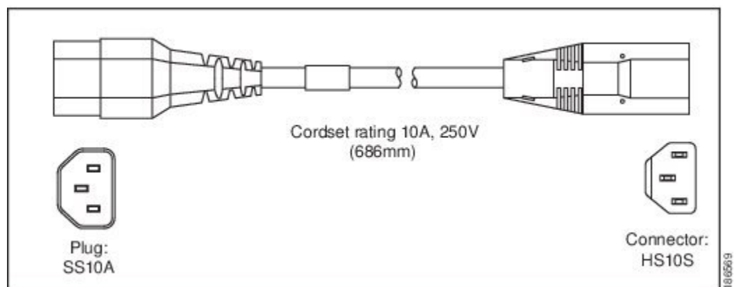
Figure 13: CAB-C13-C14-2M, Jumper Power Cord (2 m)
