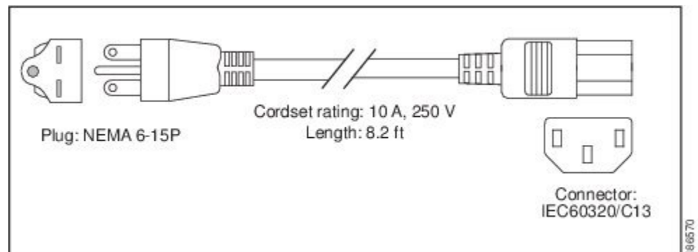
Figure 12: CAB-C13-CBN, Jumper Power Cord (0.68 m)
