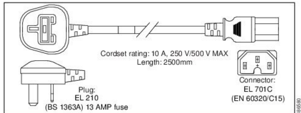
Figure 10: CAB-AC-250V/13A
