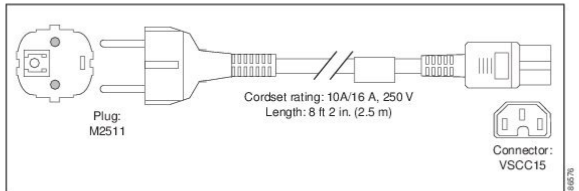
Figure 5: SFS-250V-10A-ID
